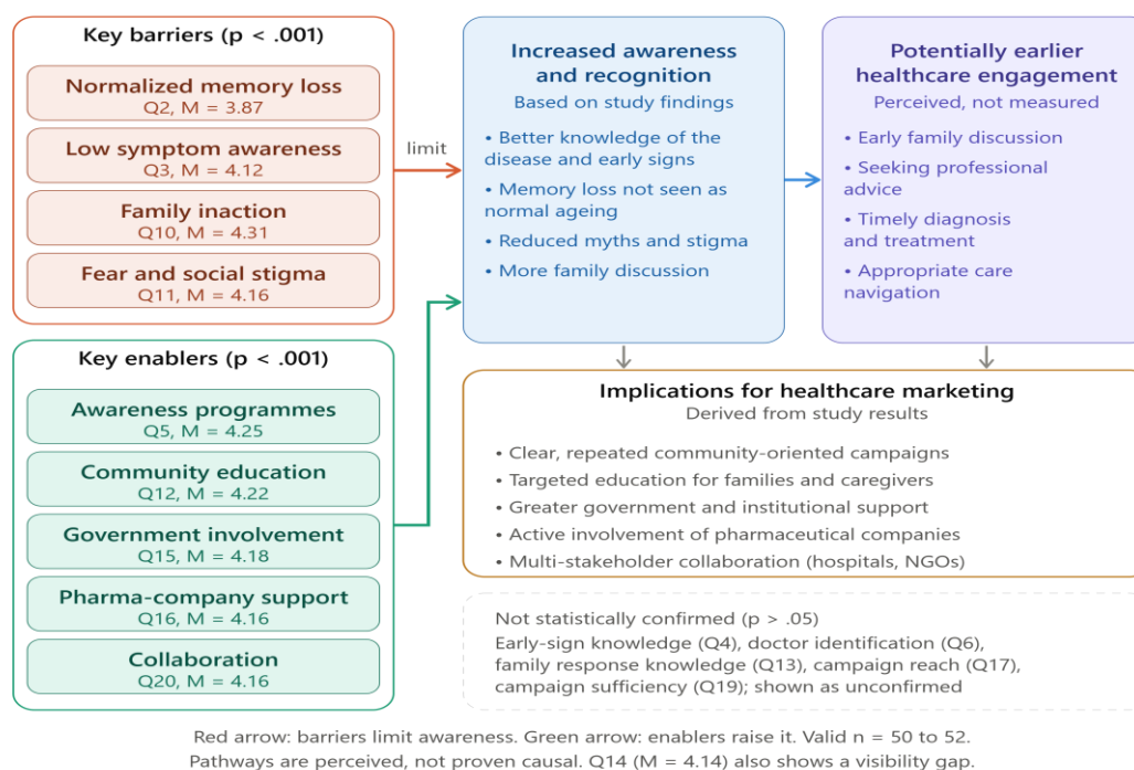
Figure 4 Finding Model
